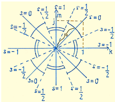
Figure 2. Complex Pythagorean rotation obtained by assigning an imaginary character to the orthogonal axis. Vanishing vector magnitude at discrete phase angles corresponds to fermionic spin measurement points ( \pm 1/2 ), while full rotation yields photon spin states (0, \pm 1 ).
