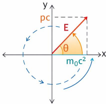
Figure 1. Geometric representation of the invariant energy relation E^2 = (pc)^2 + (m_0c^2)^2 , interpreted as a rotating energy vector with orthogonal rest-energy and momentum-energy components.
