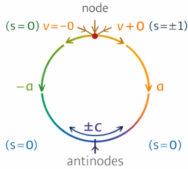
Figure 3. geometrically summarizes the alternating dynamical phases of the fermion during the Reverse Higgs transition.
