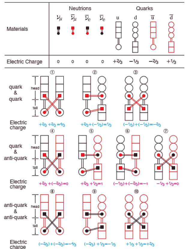
Fig.1 Combinations of quarks and anti-quarks mediated by neutrinos.
