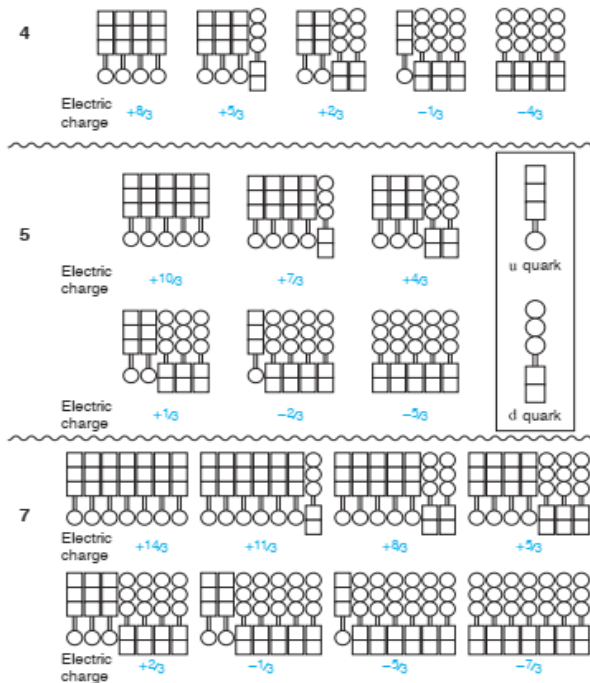
Fig. 4 Electrical charge of combinations of four, five and seven quarks.
