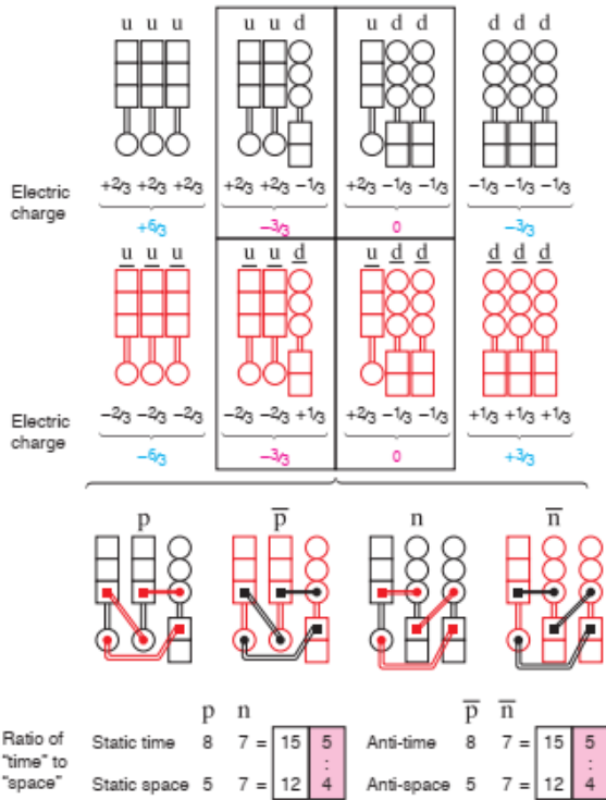
Fig. 3 Particle groups formed when three quarks and three anti-quarks combine.
