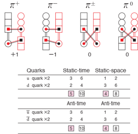
Fig. 2 Particle groups formed when two quarks and two anti-quarks combine.
