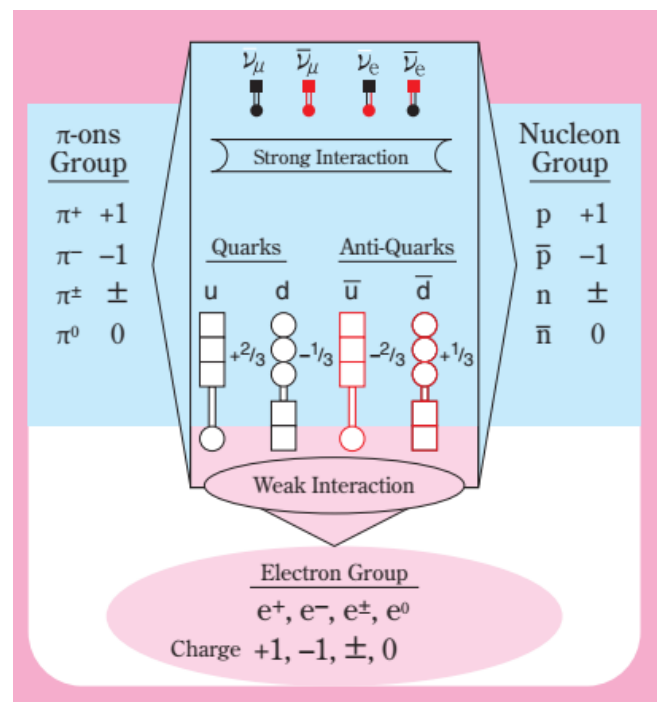
Fig. 3 (120 kinds of Elements) Further development of quarks/anti-quarks. Without any problems, it was possible for the quarks/anti-quarks ( u/\bar{u} , d/\bar{d} ) that formed to through "strong interaction" mediated by 2 pairs of neutrinos ( \nu_\mu/\bar{\nu}_\mu , \nu_e/\bar{\nu}_e ) construct the \pi -on group ( \pi^+ , \pi^- , \pi^\pm , \pi^0 ) and nucleons/antinucleons ( P , \bar{P} , n , \bar{n} ) having electrical charge composition of (+1, -1, 0, 0) . In addition, there was not even the slightest contradiction in the later creation of 120 types of atomic nuclei/anti-atomic
