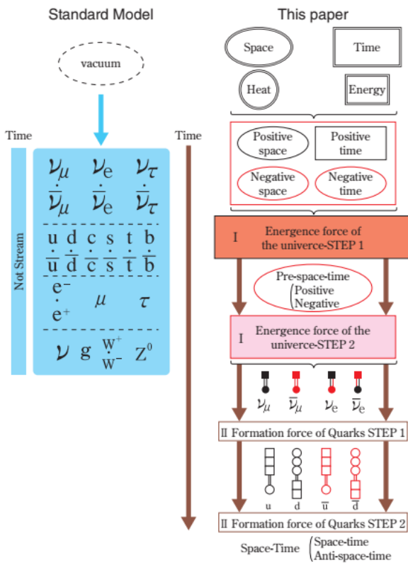
Fig. 5 Chronology of time. Due to the fact that the "main body of time" is the development of the causality of the entire universe, time passed and pre-space-time/anti-pre-space-time, neutrinos, space-time/anti-space-time, and quarks/anti-quarks were formed due to the acting of causality such as the "emergence force of the universe" and the "formation force of quarks." On the other hand, the "vacuum phase transitions" of the Standard Model are not causal phenomena, so it is not possible for "time," which forms neutrinos and quarks/anti-quarks, to flow.
