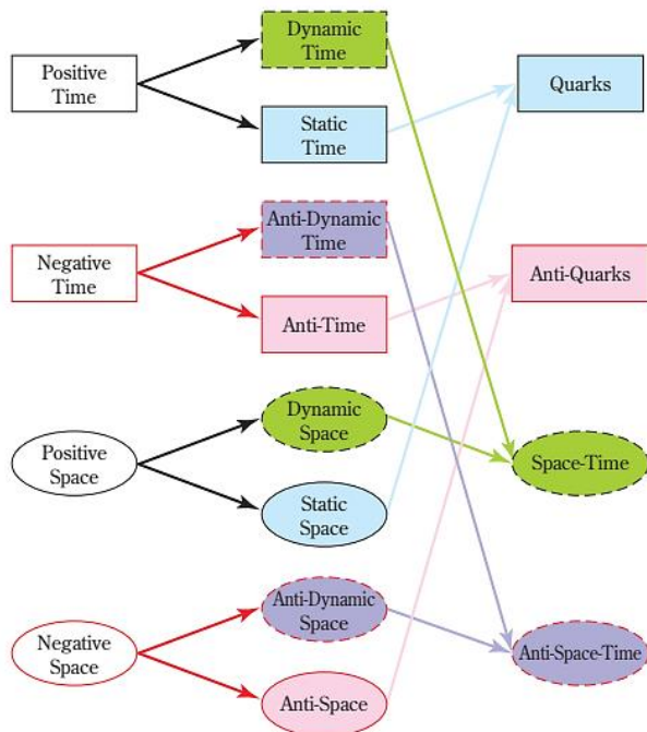
Fig. 1 Positioning of the quarks/anti-quarks in the entire universe Half of the 4 entities starting with "positive time" remaining from the formation of pre-space-time/anti-pre-space-time and neutrinos were separated into halves and formed space-time/anti-space-time and quarks/anti-quarks.
