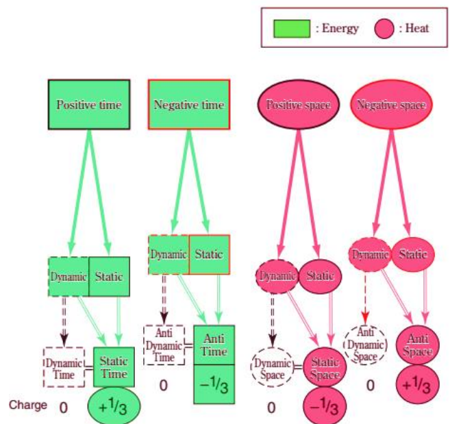
Fig. 2 Separating the 4 entities starting with "positive time" into 4 types of "dynamic" and "static" entities. The 4 entities starting with "positive time" were separated into 4 types of "dynamic" and "static" entities. The "energy" and "heat" contained within the 4 "dynamic" entities transitioned to the 4 "static" entities and became their electrical charges.
