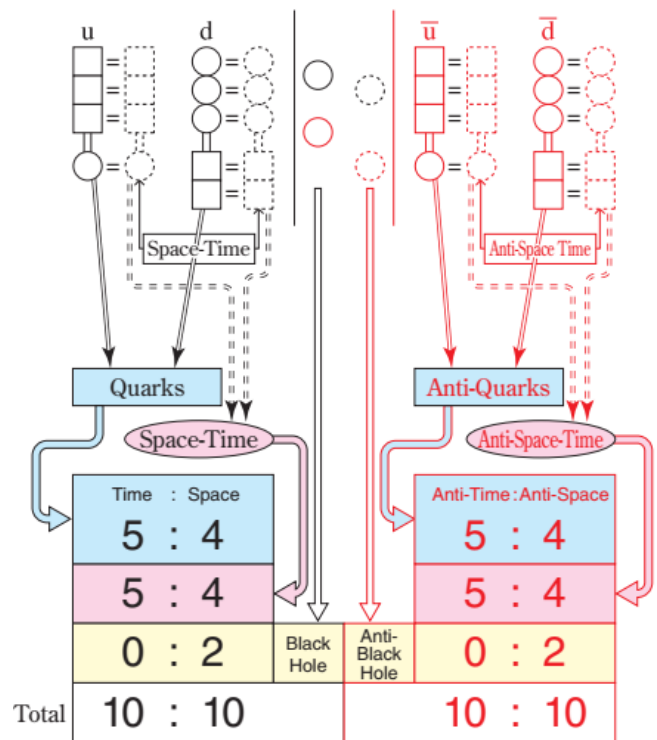
Fig. 4 Component ratios of "time" to "space" for quarks/anti-quarks and space-time/anti-space-time. The component ratios of "time" to "space" for both quarks/anti-quarks and space-time/anti-space-time are 5:4. Positive and negative "black holes" formed from the remaining 2 pairs of positive and negative "space" entities.
