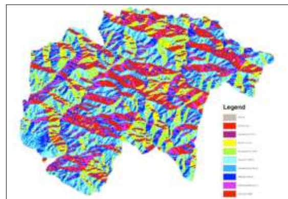
Figure 4: Aspect map considered area
