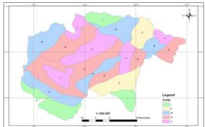
Figure 6: The map of landslide hazard zonation provided in fuzzy way model
