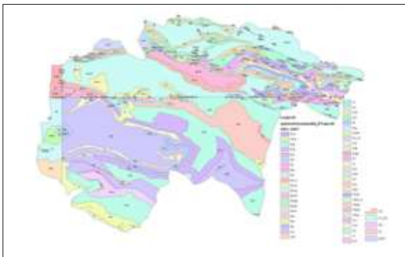
Figure 2: The geological map of considered area Material and Methods
