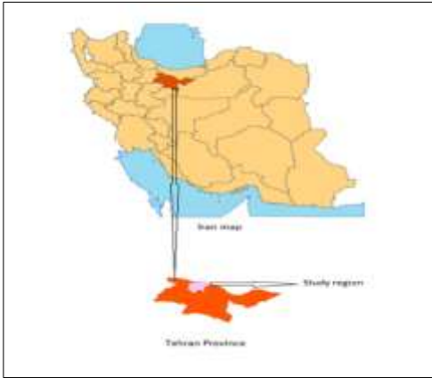
Figure 1: Geography Location map of study area
