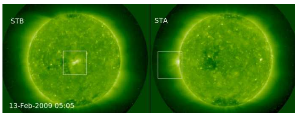
Images of the Sun from the STEREO Behind ("STB") and Ahead ("STA") spacecraft's SECCHI Extreme Ultraviolet Imager (EUVI) instrument, obtained on February 13, 2009, in a spectral line formed at 1.5 million Kelvin. The spacecraft orbit the Sun just inside (Ahead) and outside (Behind) the earth's orbit; in February, they were 90° apart, so Behind was able to observe the boxed active region nearly at disk center, while Ahead saw it on the limb, or edge of the Sun. STEREO - Planet identification in STEREO coronagraph images
