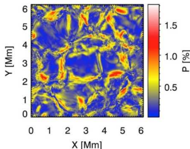
Fractional total polarization signals of the Sr I 460.7 nm line predicted for the disk center line of sight in the model of the quiet solar photosphere / Credit: del Pino Alemán et al. (2018; ApJ) .
