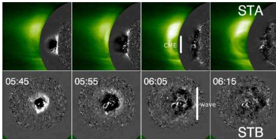
STEREO Ahead ("STA") and Behind ("STB") views of the coronal wave event. The Behind spacecraft views ( bottom ) show the wave expanding over much of the solar hemisphere visible from that spacecraft, while the Ahead spacecraft ( top ) shows the expanding coronal mass ejection (CME) bubble leaving the EUVI field of view (grey difference images) and entering the COR1 field of view (green images). STEREO - Planet identification in STEREO coronagraph images
