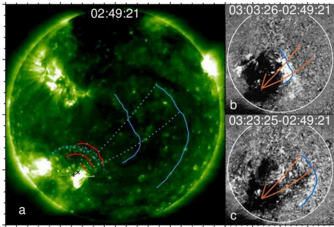
"EUV wave (blue) and Moreton wave in the 24 September 1997 event. a) Non-subtracted EIT 195Å image with the first front (blue crosses). Blue dotted line outlines its foremost edge. Red fronts outline the Moreton wave. White broken lines trace the measurement great circles. Black crosses denote the origins of measurements. b,c) Difference ratio images with blue outlines of EUV wave fronts and red measurement great circles. The outlines correspond to Warmuth et al., 2004a (courtesy A. Warmuth)."
