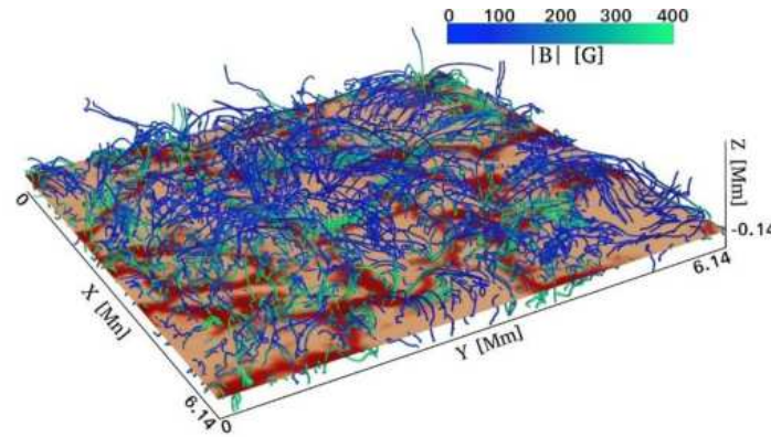
Conceptual of the magnetic field in a 3D magneto-convection model of the quiet solar photosphere (Rempel 2014; ApJ 789, 132), which has a surface mean field strength of 170 gauss. Credit: Del Pino Alemán et al. (2018)
