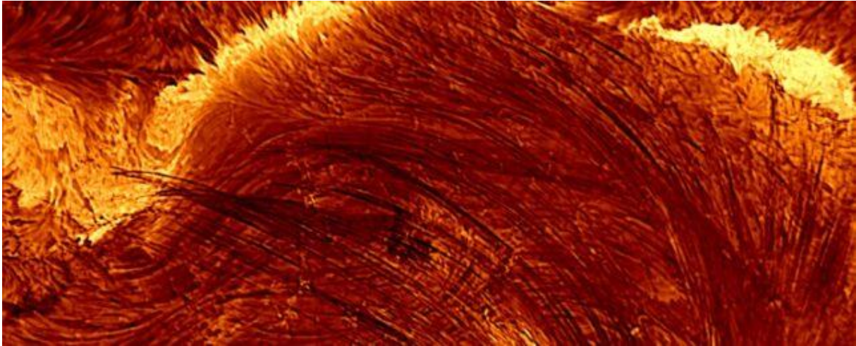
This is the highest resolution at which we've ever seen a solar flare. ( NSF/NSO/AURA )
